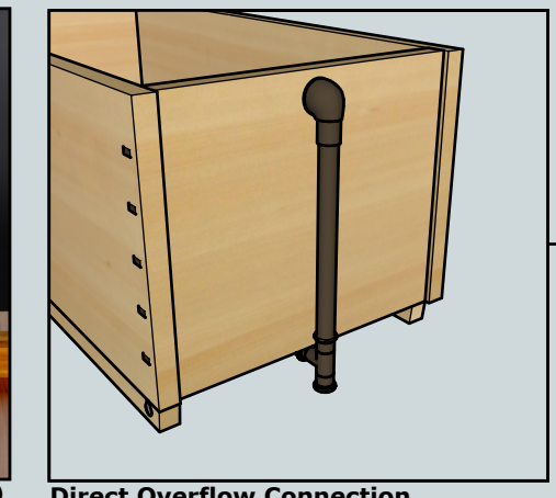
Direct Overflow Connection 1-1/2" Slip Joint
