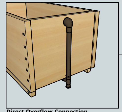
Direct Overflow Connection 1-1/2" Slip Joint
