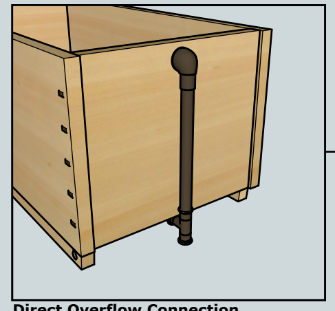
Direct Overflow Connection 1-1/2" Slip Joint
